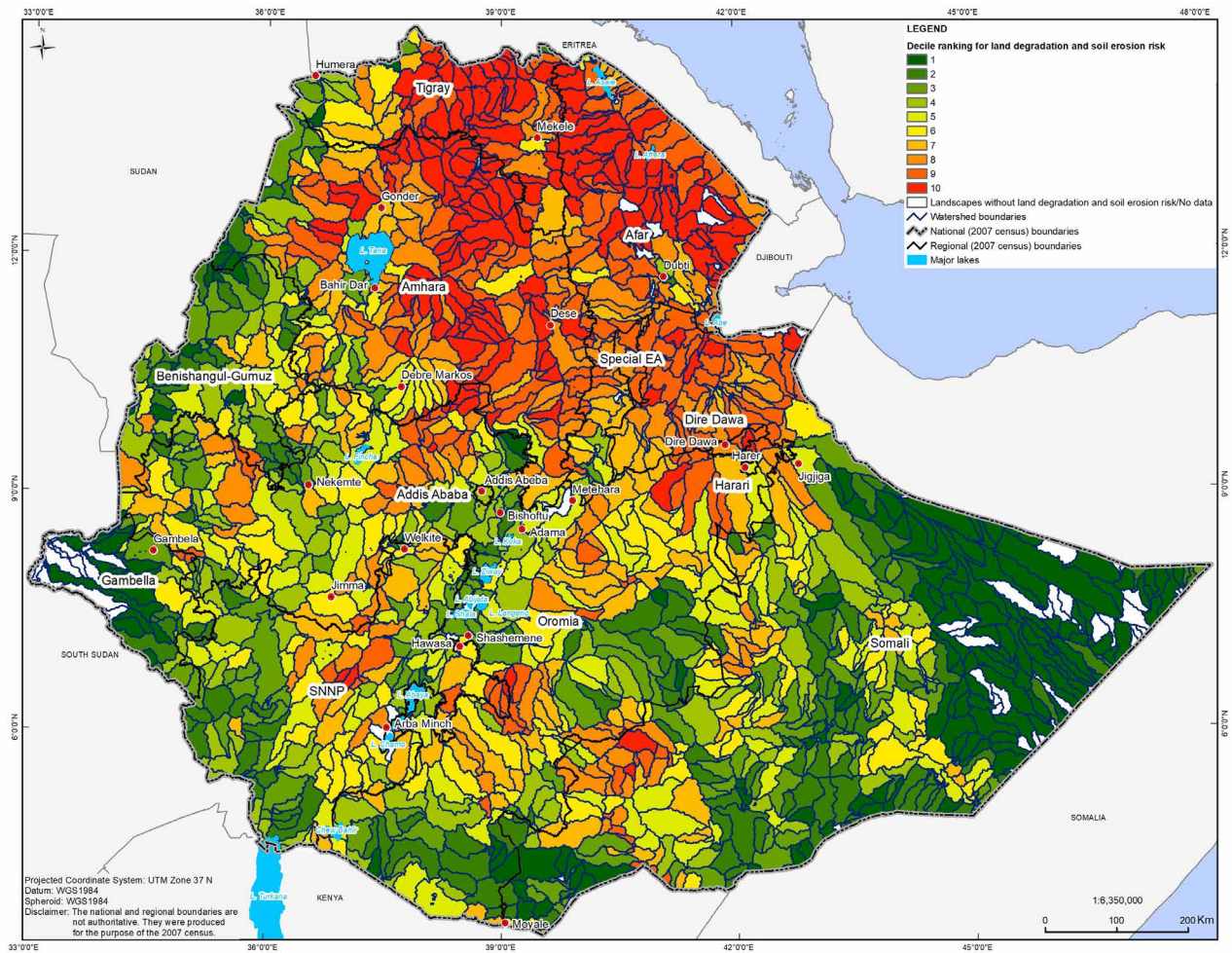
CAPTION: Map 4b shows the decile ranking of landscapes based on their average land degradation, where each class contains approximately 10 percent of the values. Landscapes in dark green are in the bottom 10 percent in terms of average land degradation, while landscapes in bright red are in the top 10 percent.
