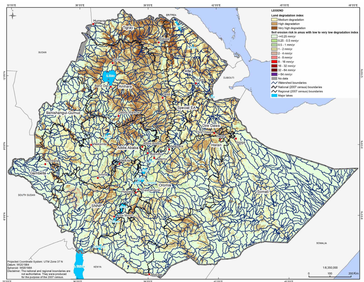
CAPTION: Map 4a shows the degradation index in areas where degradation can be observed and soil erosion risk in areas where degradation has not yet taken place. The degradation index is based on vegetation index, rainfall erosivity, soil erodibility, slope aspect, and human and livestock population density (Wangui 2013). The degradation index goes from medium (in beige) to high (in brown) and very high (in dark brown). Soil erosion risk is based on the combined effect of rainfall, soil factor, slope length, slope gradient, land cover factor, and land management factor (MoARD 2004). Soil erosion risk varies from very low (in light green) to very high (in purple). Erosion can occur and yet permit crop productivity to be sustained economically if it is at a rate below 1 mm of soil depth/year (Montgomery 2007). Consequently, only areas with soil erosion risk above 1 mm of soil depth/year (from tan to dark brown) were considered of interest in later steps of the prioritization process.
