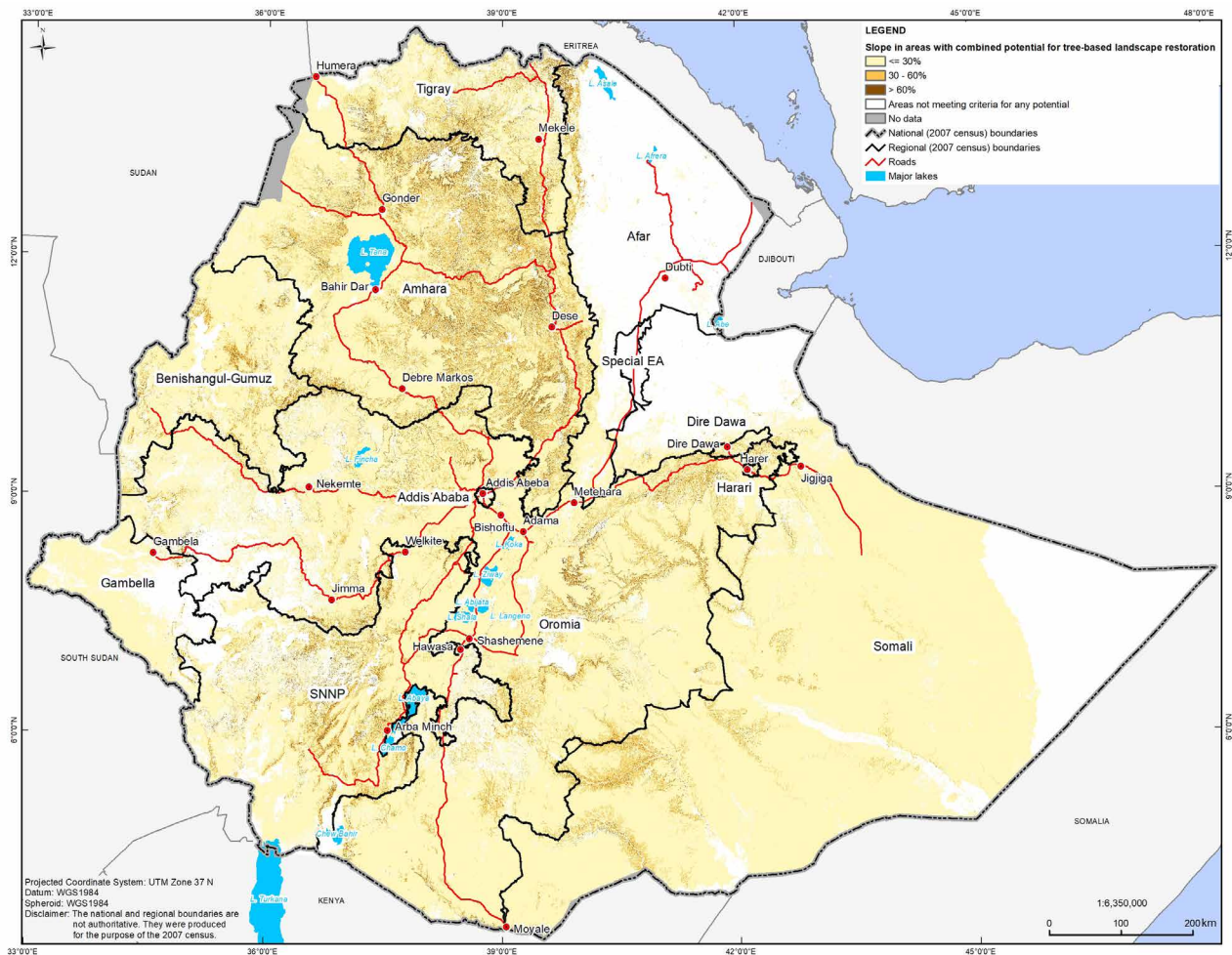
CAPTION: Map 1c shows the slope in areas with combined potential for tree-based landscape restoration. Most areas are on slopes below 30% (in salmon). Some areas are on slopes between 30 and 60% (in orange), and few are on slopes over 60% (in brown). Slope steepness will dictate the type of soil and water conservation measures to be implemented as per the Federal Rural Land Administration and Use Proclamation (FDRE 2005). Slope can also be a consideration in terms of the type of ecosystem services to which trees can contribute. For example, trees and forest in areas with steep slopes would contribute most to preventing soil erosion and landslides.
